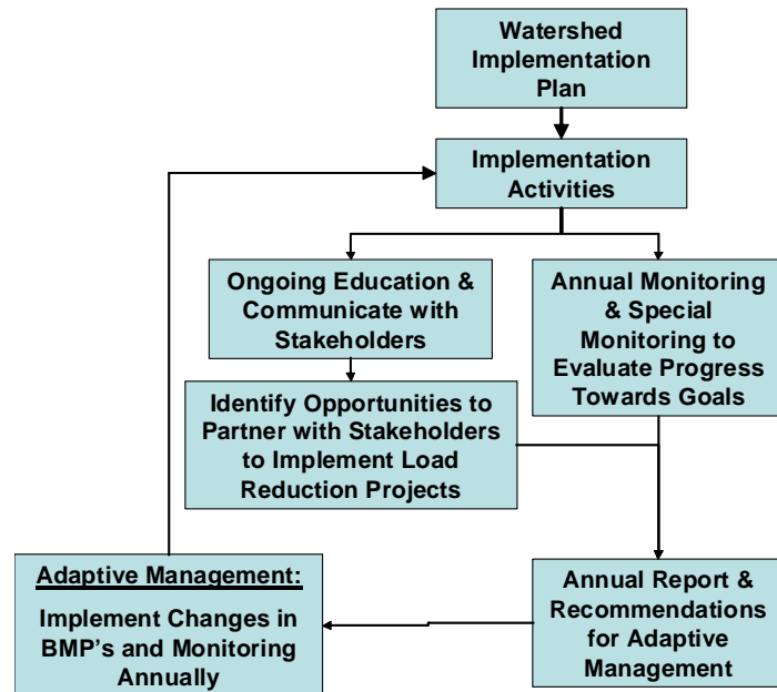
Figure 11.1 Implementation Framework
